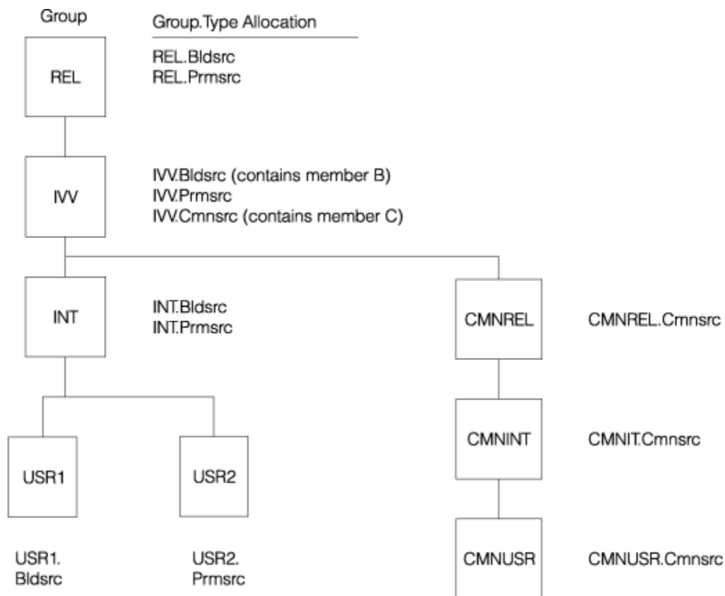
Figure 8. Invalid Hierarchy for Intended Operation
