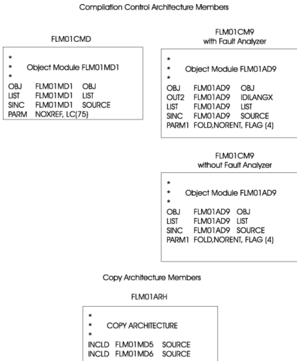
Figure 150. Architecture Members for Application Sample FLM01AP1 (Part 2 of 2)
