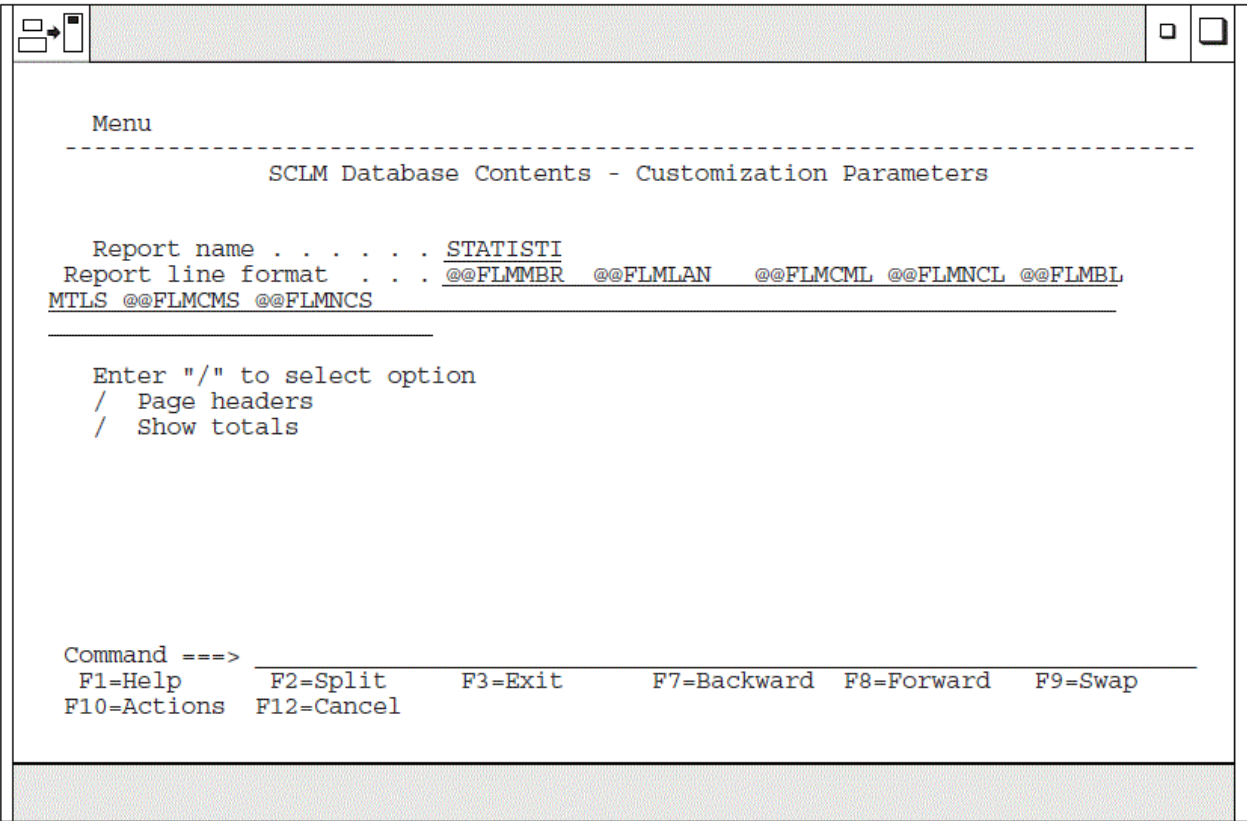
Figure 89. SCLM Database Contents - Customization Parameters (FLMRCT)
