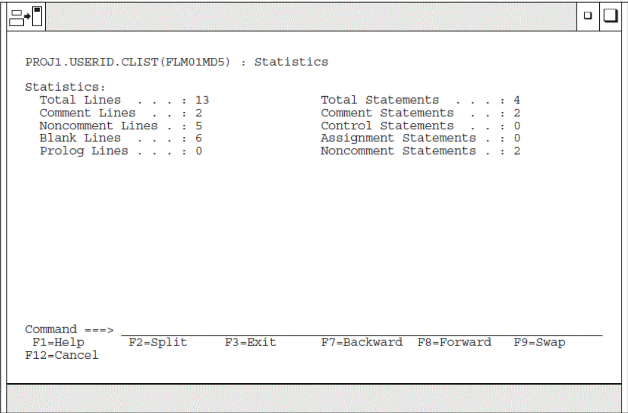
Figure 76. Accounting Record Statistics (FLMUSS#P)
