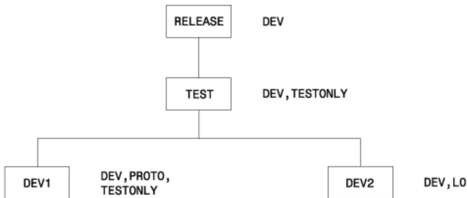
Figure 6. Sample Hierarchy with Authorization Codes
