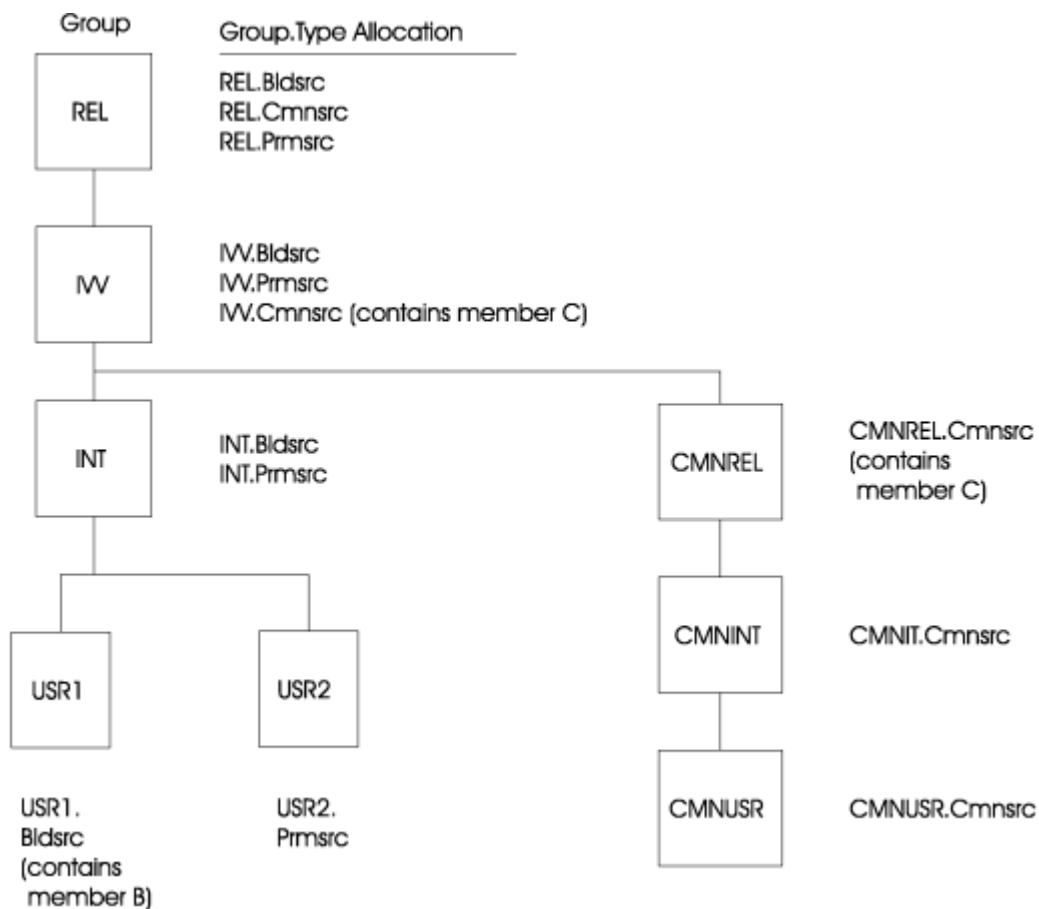
Figure 7. Valid Hierarchy with Unallocated Data Sets
