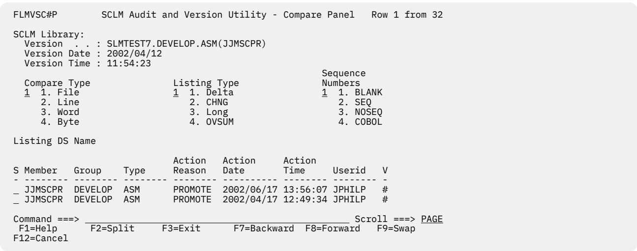
Figure 112. SCLM Audit and Version Utility - Compare Panel (FLMVSC#P)
