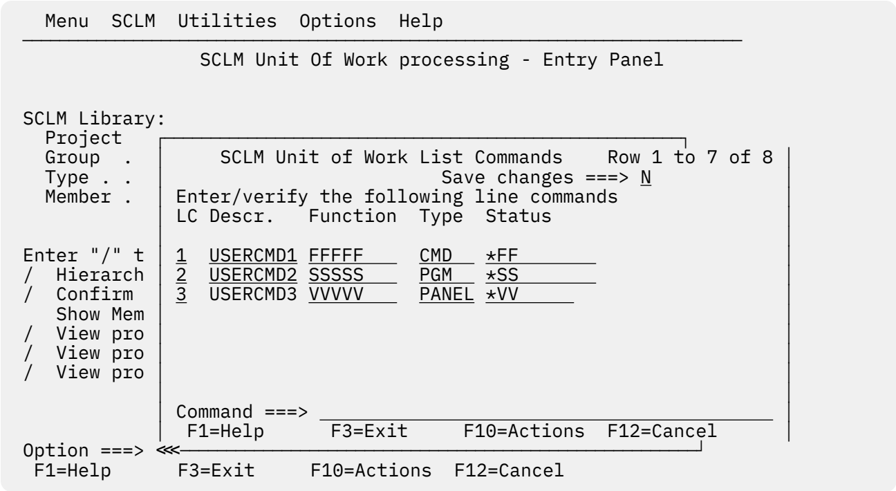
Figure 125. SCLM Unit of Work List Commands panel
