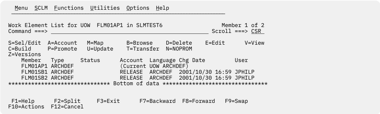
Figure 127. Work Element List panel
