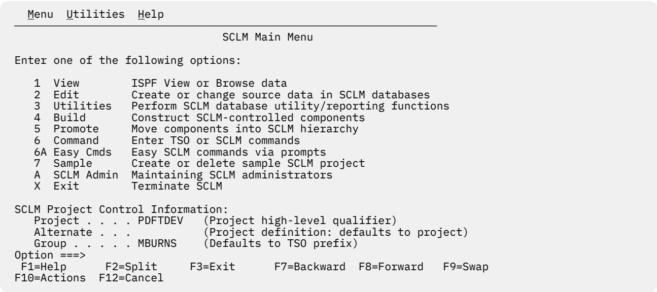
Figure 67. SCLM Main Menu Panel (FLMDMN)
