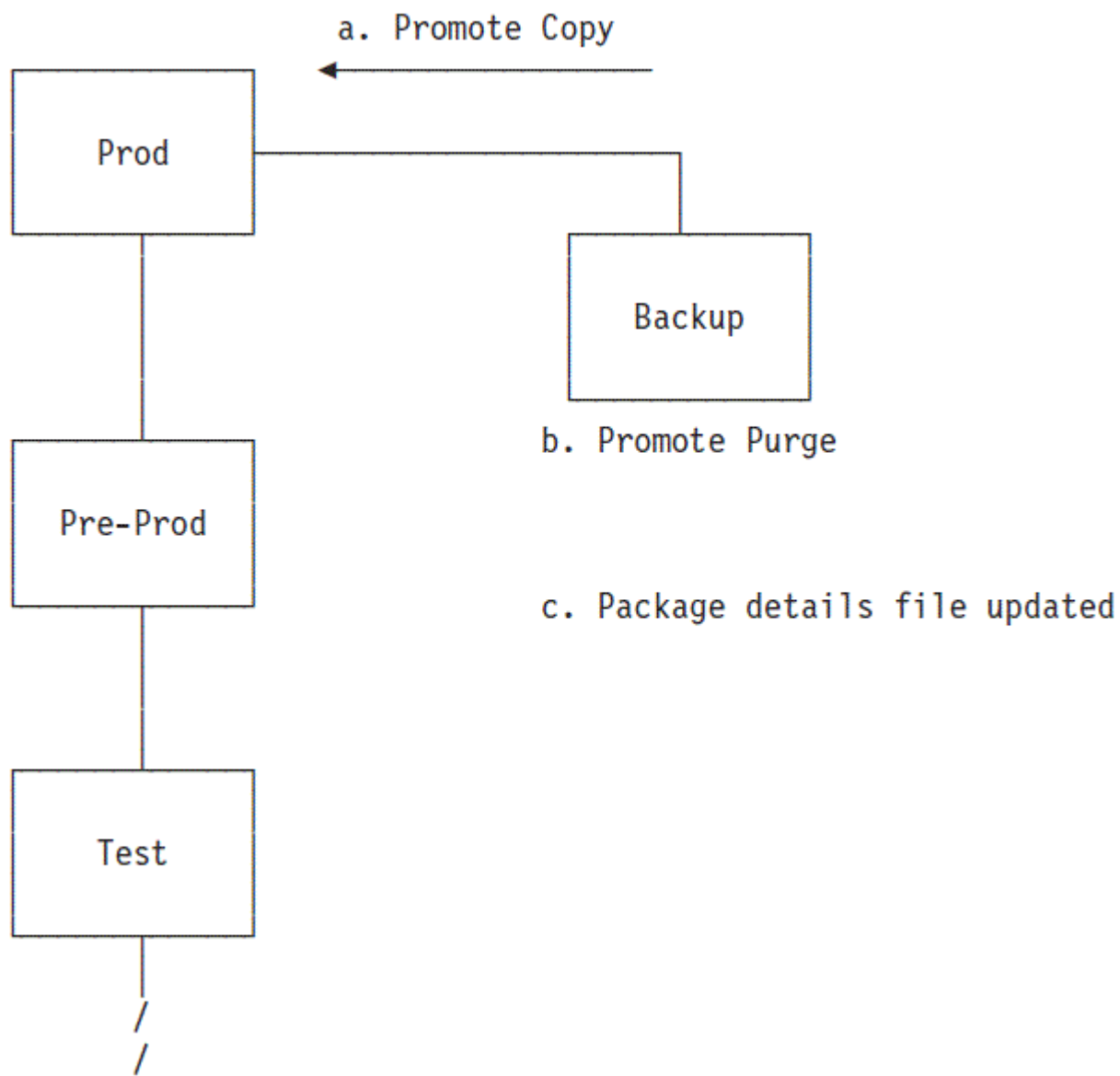
Figure 118. Package Backout—Restore Phase
