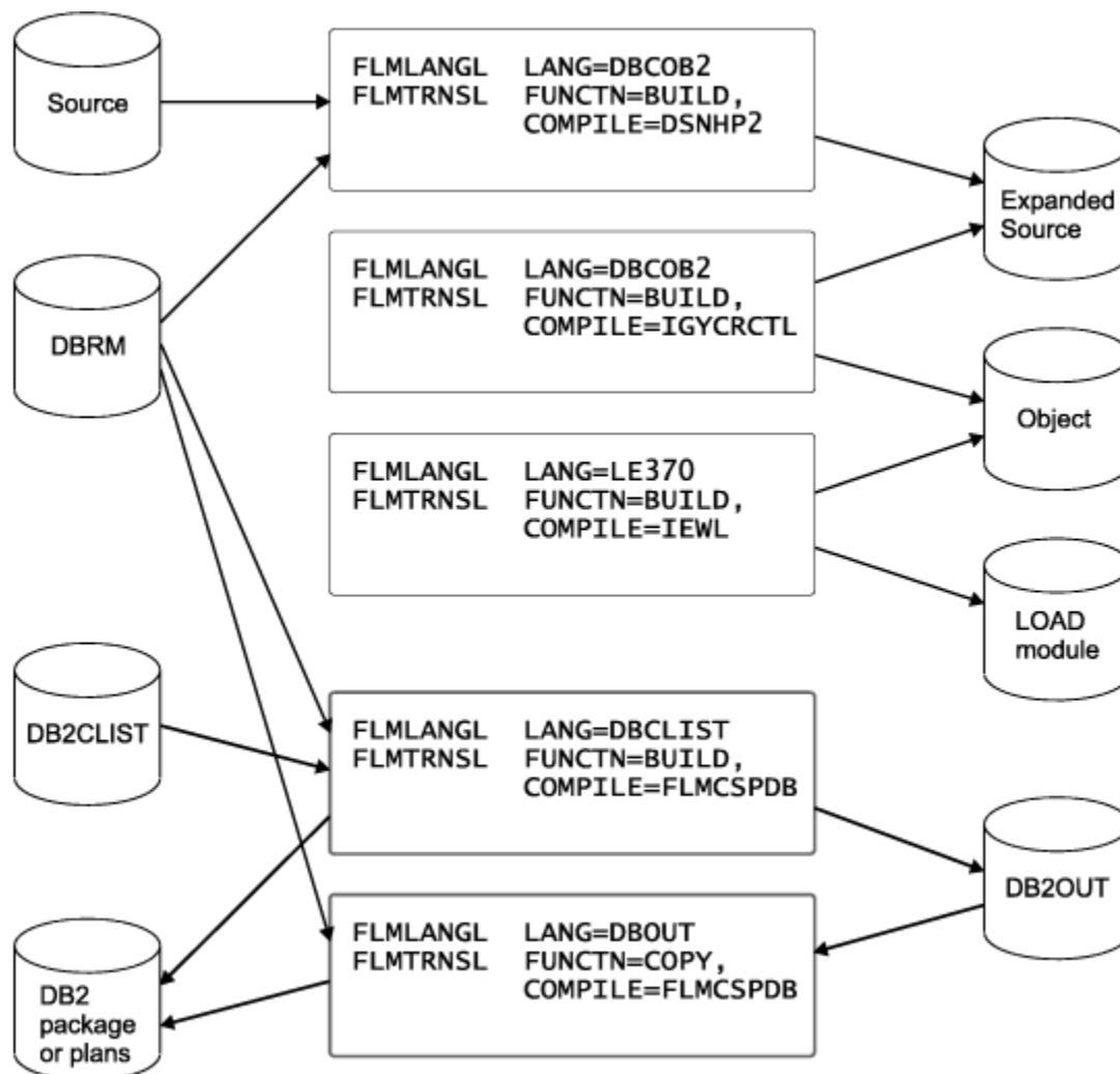
Figure 155. DB2CLIST: flow of processing through the translators
