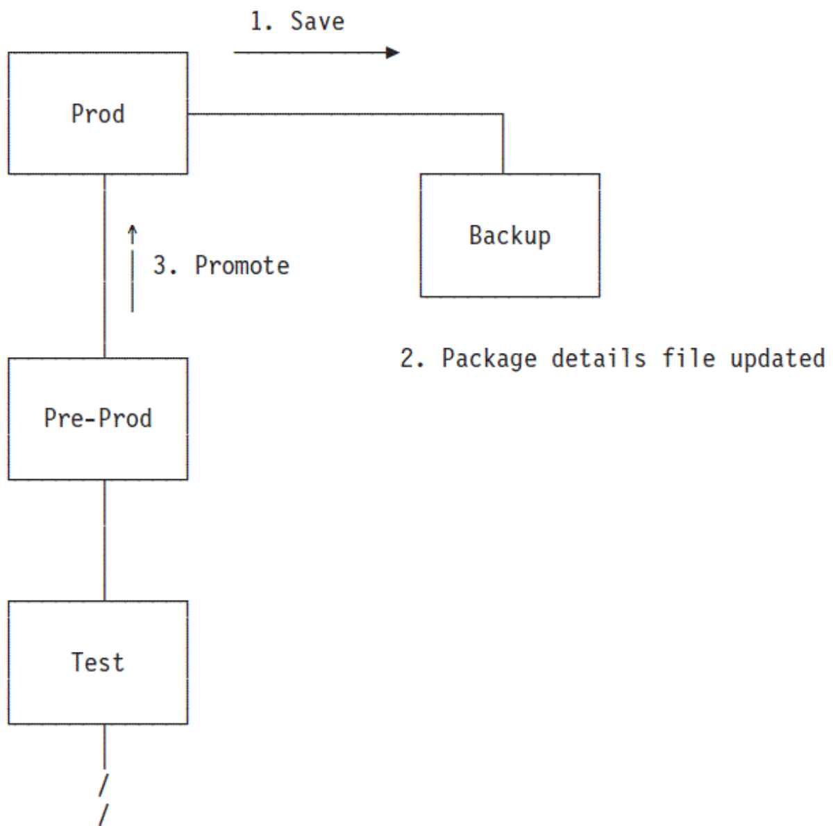
Figure 117. Package Backout–Backup Phase
